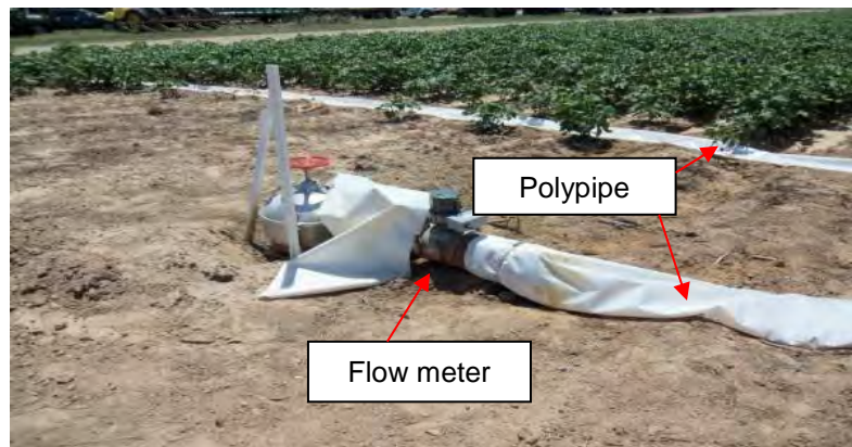
Photo 7. An in-line, turbine type flow meter to measure application volumes and the polypipe distribution system.
